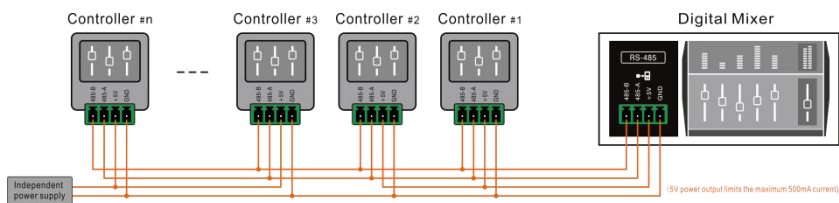
Wiring diagram of 86 box wallboard controller
